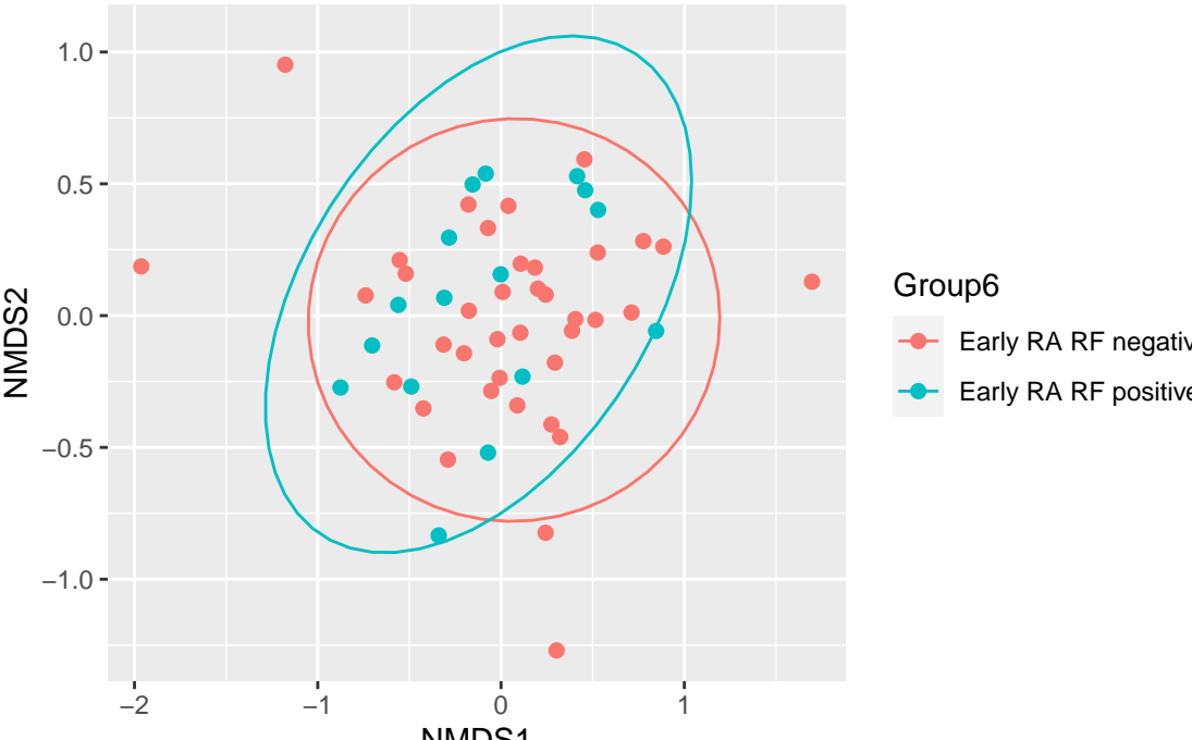
NMDS Plot with Bray–Curtis Dissimilarity Metric
